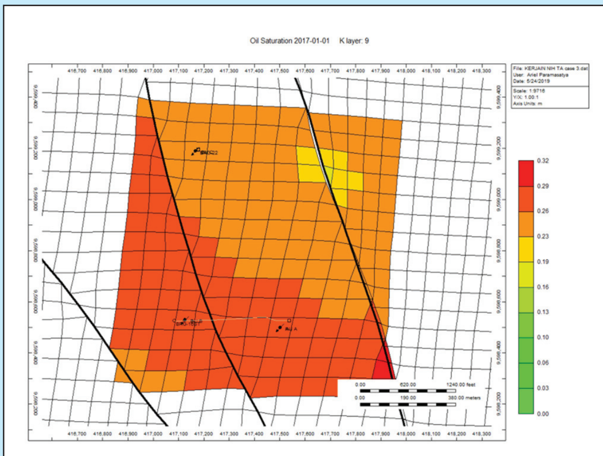
Figure 1 Model reservoir of X field.
