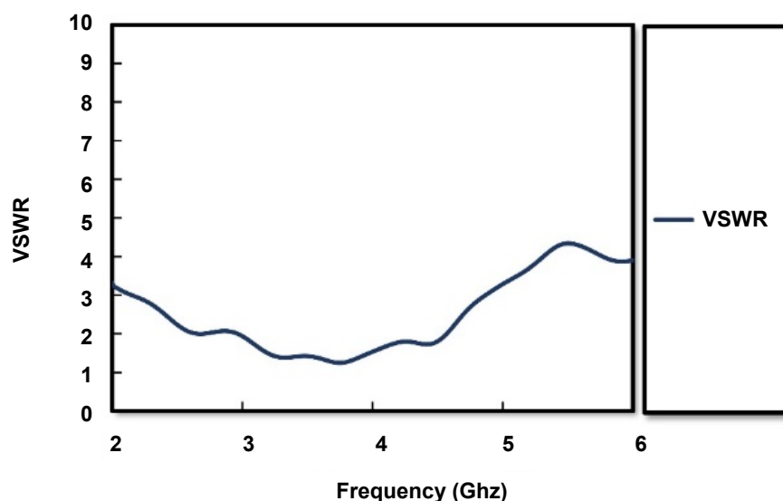
Figure 5. Voltage Standing Wave Ratio (VSWR) of the final 2×2 Multiple-Input Multiple-Output (MIMO) antenna design.
