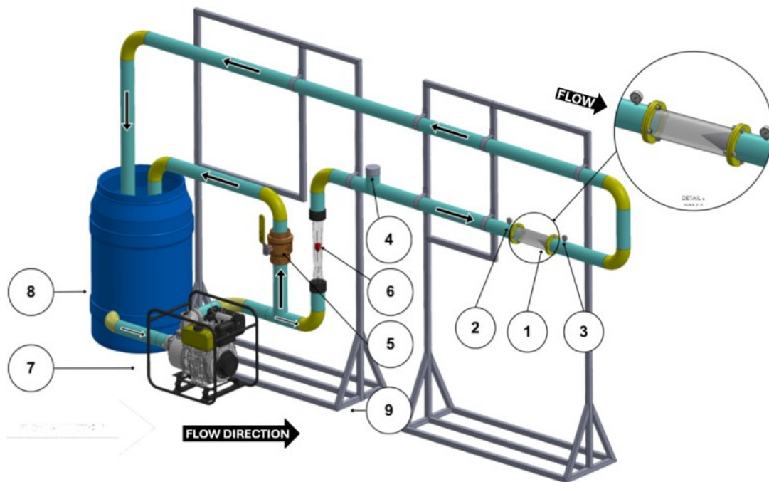
Figure 1. Experimental setup
