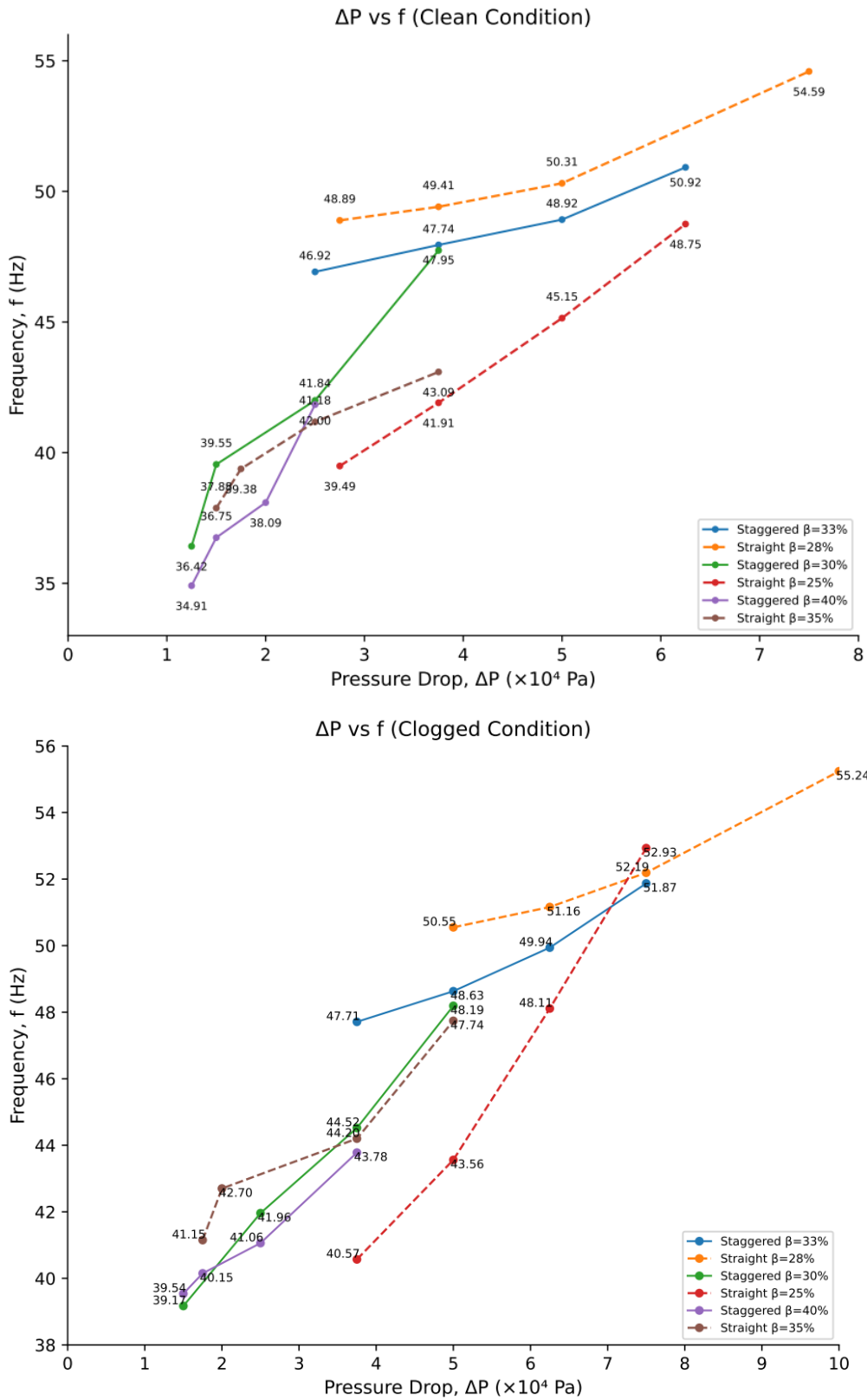
Figure 6. The effect of \beta and \Delta P to f under clean and clogged conditions. The \Delta P - f relationship under clean and clogged conditions shows an increase in vibration frequency with increasing pressure drop, with a stronger dynamic response under clogged conditions.
