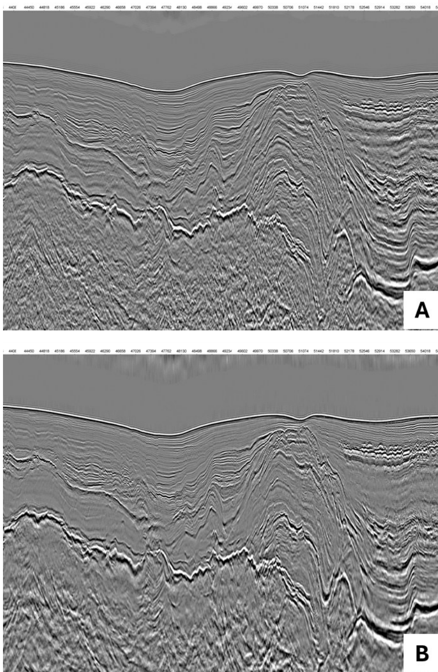
Figure 6. An example of real data of the conventional PSTM gather (A), and PSTM CO-CRS gather (B) stack section.
