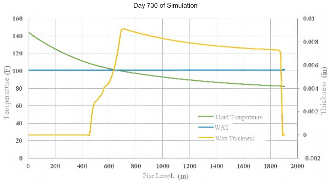
Figure 9. . Temperature and wax thickness distribution along the pipeline after 730 days of simulation. The fluid temperature (green) gradually decreases along the pipe and falls below the Wax Appearance Temperature (blue), leading to noticeable wax deposition (yellow) particularly after the cooling point, indicating zones vulnerable to wax buildup due to thermal losses.
