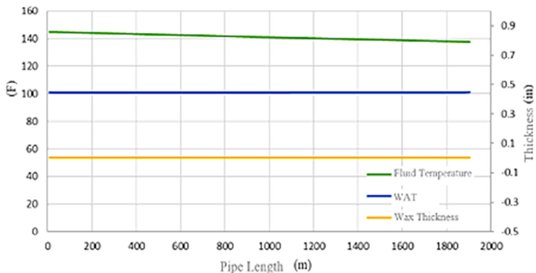
Figure 5. Temperature and wax thickness profile along the pipeline after 730 days of operation with polyurethane insulation. The fluid temperature (green) remains above the Wax Appearance Temperature (blue), resulting in minimal wax layer buildup (orange), indicating effective thermal retention by polyurethane.
