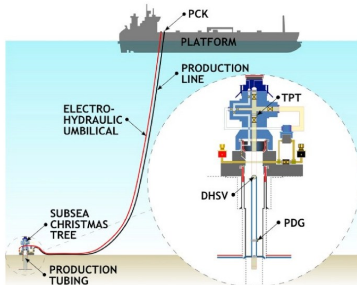
Figure 1. Schematic of the offshore production system in 3W Dataset, depicting the subsea Christmas tree, production tubing, electro-hydraulic umbilical, and production line connected to the platform. The figure also shows the locations of critical sensors for this study, including PCK, TPT, PDG, and DHSV. (Vargas et al., 2019)
