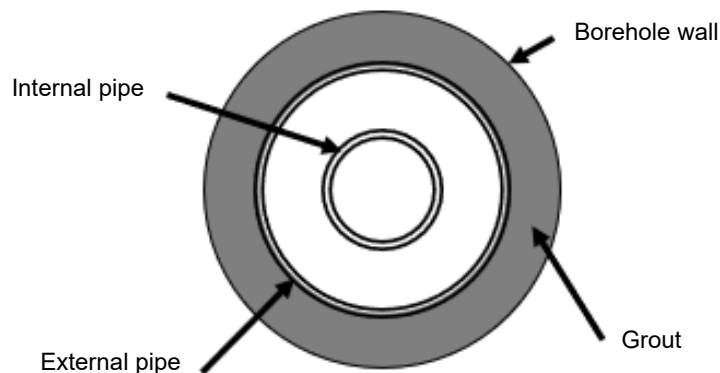
Figure 3. Cross section of coaxial double-pipe heat exchanger.
