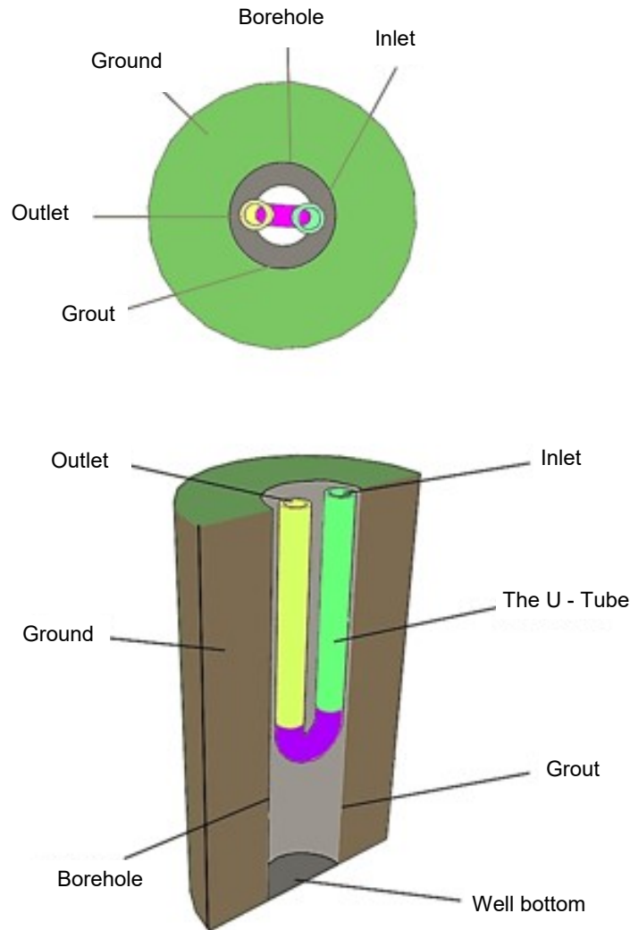
Figure 2. Schematic diagram of an underground single-pipe U-pipe heat exchanger.
