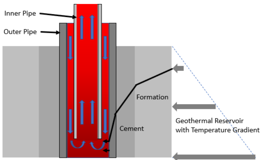
Figure 1. Schematic illustration of heat transfer and fluid flow in a double-pipe heat exchanger system. The working fluid flows downward through the outer pipe and upward through the inner pipe, enabling counter-current heat exchange with the surrounding geothermal reservoir through the cemented wellbore and formation.
