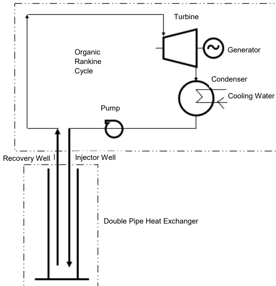
Figure 4. Geothermal power plant structure diagram.
